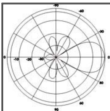
Horizontal Plane
